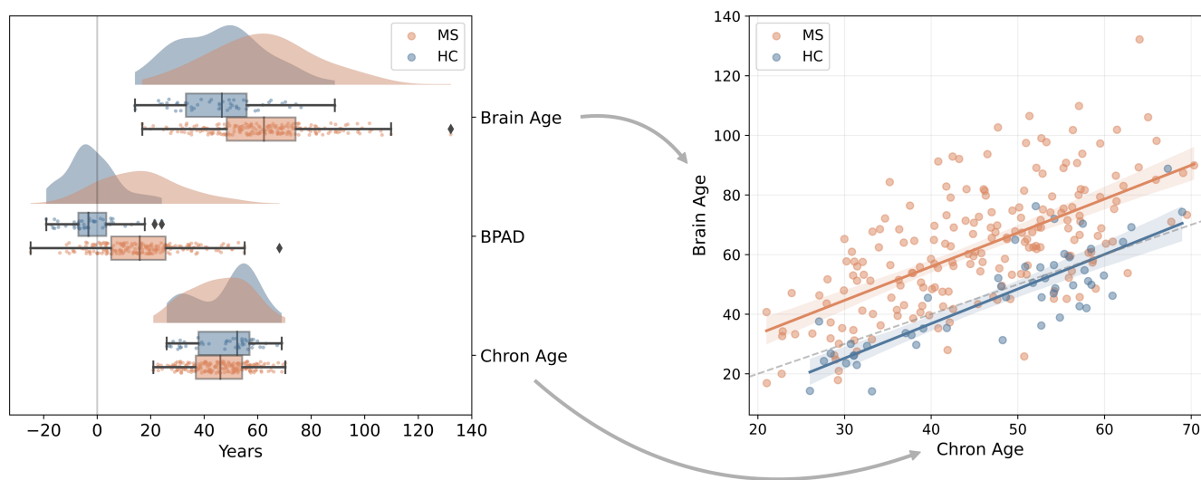
FIGURE 2 Group comparison between HC_test (blue) and MS_test (orange) for brain age, BPAD and chronological age. Left: The raincloud plots show the distribution of brain age, BPAD and chronological age for MS_test and HC_test. A reference line at x = 0 is included as visual aid. Right: The scatterplot shows the relationship between brain age and chronological age for MS_test and HC_test. The dotted line is added as reference, namely where brain age = chronological age [Colour figure can be viewed at wileyonlinelibrary.com ]
