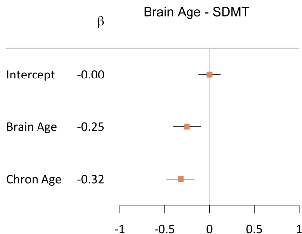
FIGURE 4 The relationship between brain age and SDMT, independent of chronological age. Left: Scatterplot between BPAD and SDMT in the MS test dataset. The textbox describes the Pearson r statistic, along with the p value. Right: Forest plot visualizing the significance of the weights ( \beta_i ) in the linear regression equation SDMT = \beta_0 + \beta_1 BrainAge + \beta_2 ChronologicalAge + \epsilon in the MS test dataset (note that variables were normalized with respect to mean and standard deviation before input in the regression equation). The maximum likelihood estimates of the weights ( \beta_i ) are represented by the orange squares, along with a 95% confidence interval (horizontal bar). If the latter does not include 0, the contribution of that feature to the model is considered significant. Brain age and chronological age contributed significantly ( p = 0.002 and p < 0.001 respectively) [Colour figure can be viewed at wileyonlinelibrary.com ]
